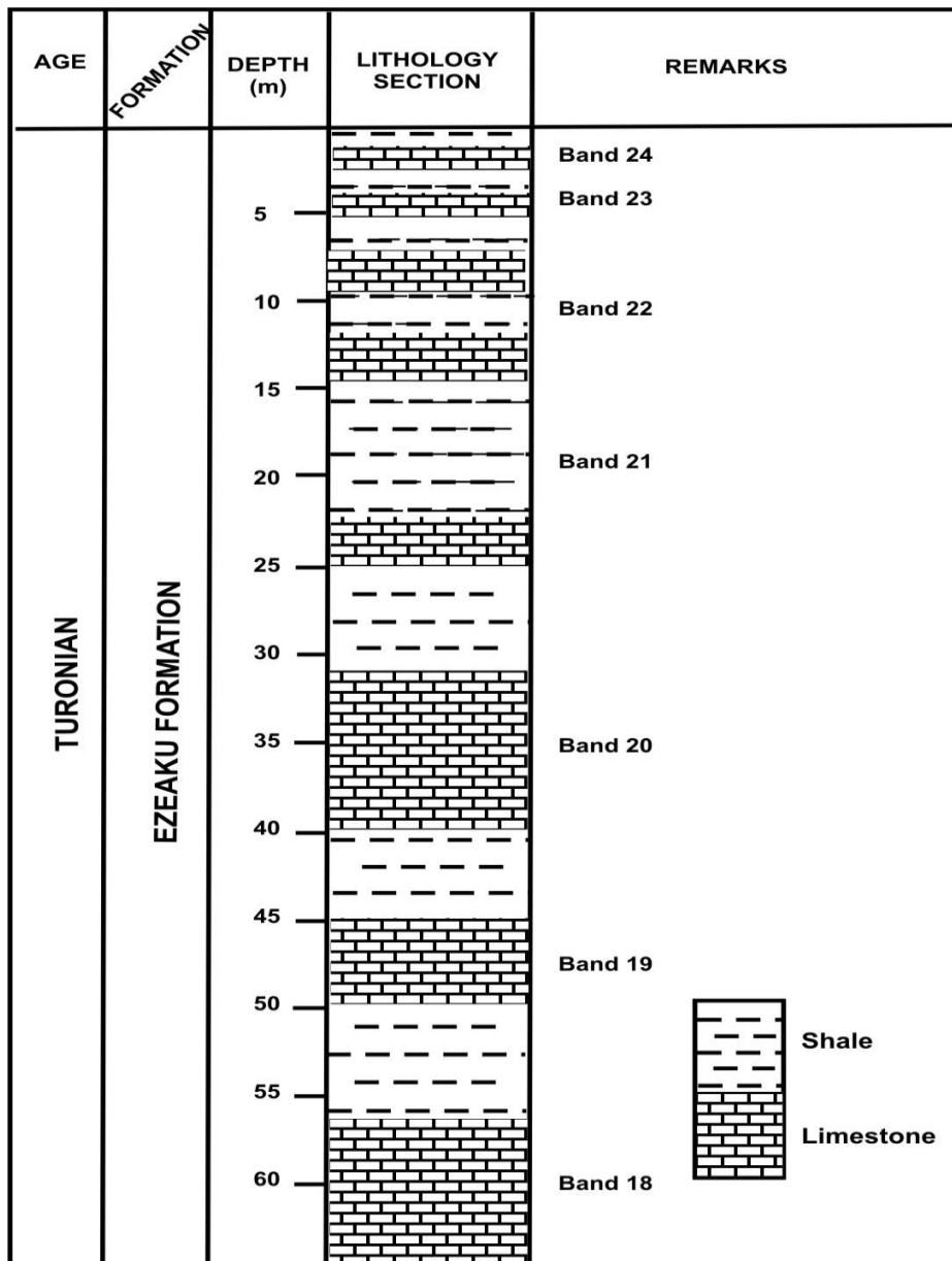
Figure 2: Typical vertical lithologic section at NIGERCEM quarry face at Nkalagu (Modified Amajor, 1992)
