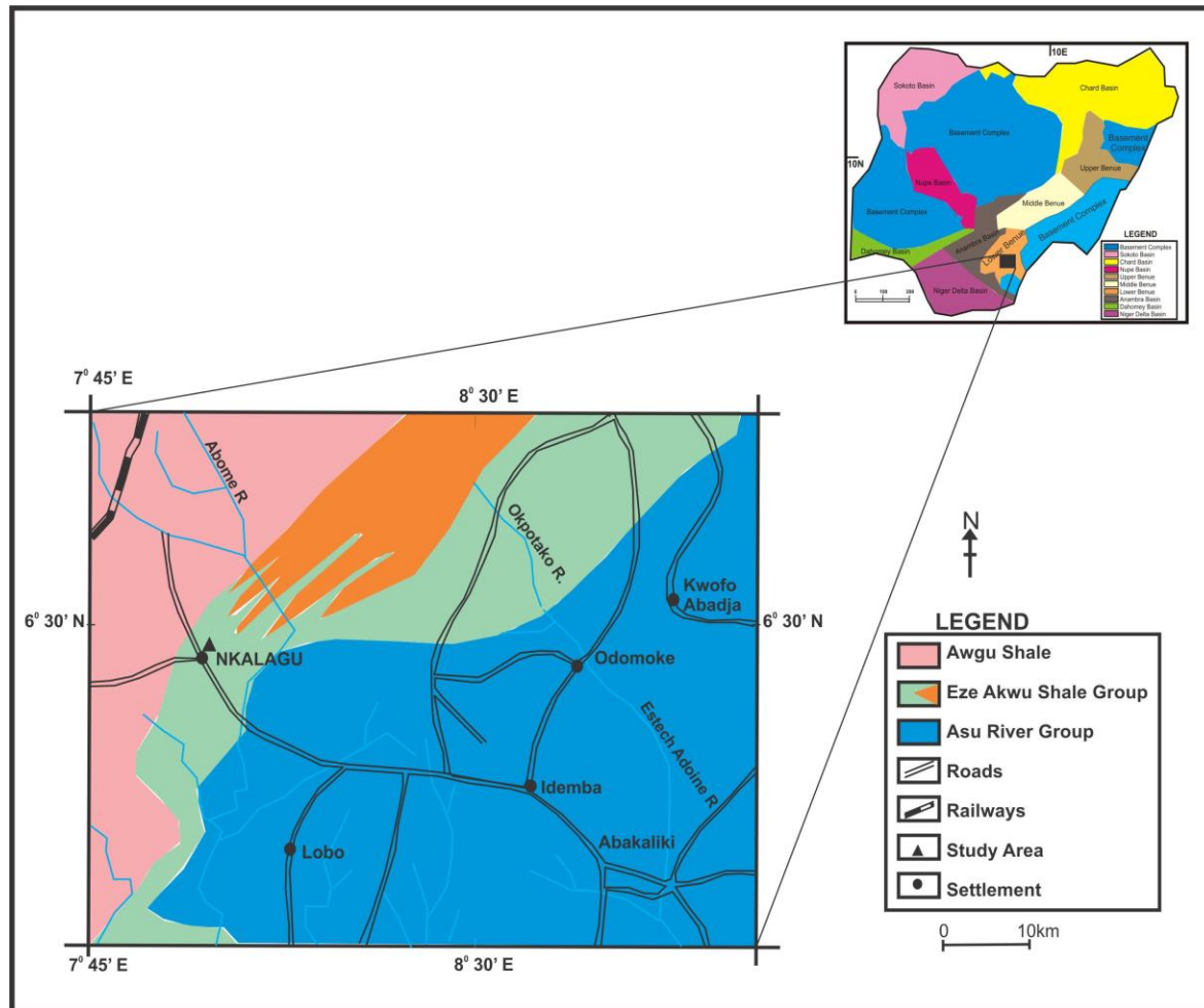
Figure 4: Geological map of Nkalagu and its environ with geological map of Nigeria (modified After Amajor, 1992)
