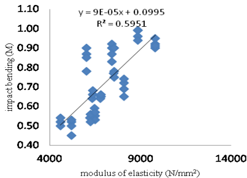
Fig. 3: Relationship between impact bending and modulus of elasticity in Vitex doniana
