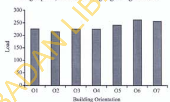
Fig. 6: Variation of building thermal load with different building orientation
