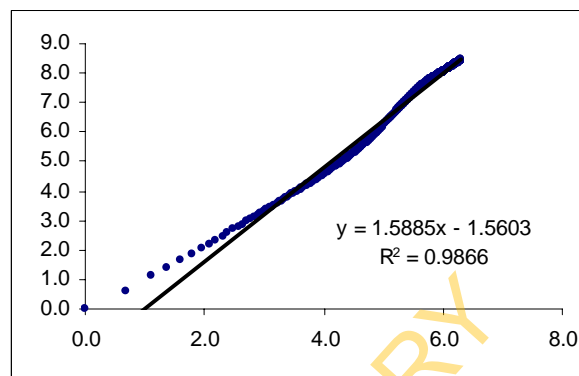
Figure 12. Log of average distance versus log of time step for case 4 in 3-D
