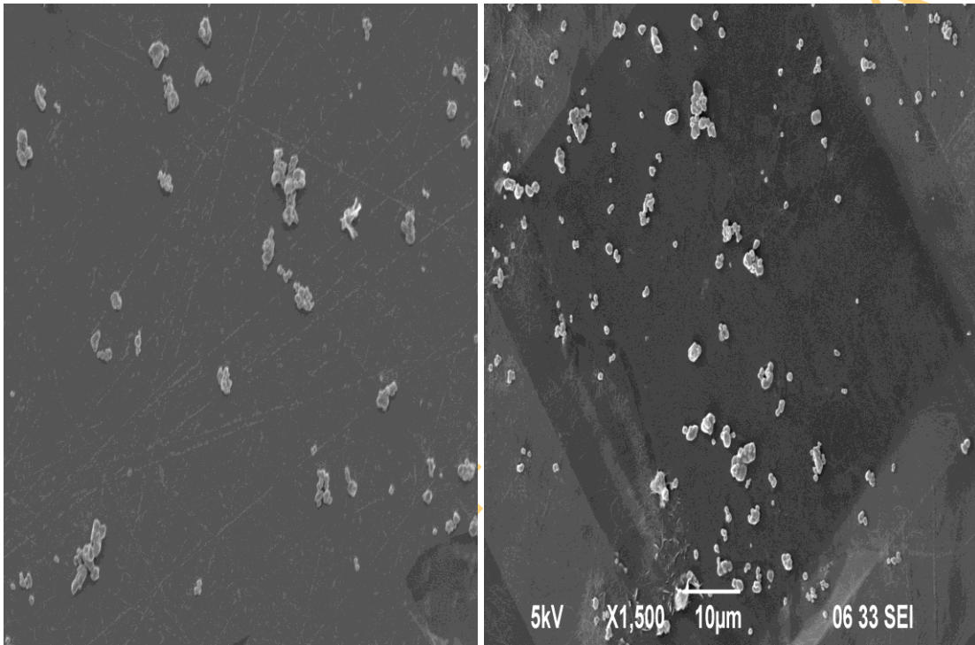
Figure 4.7: Electron micrographs showing the effect of sonication on BaCrO 4 particles.
