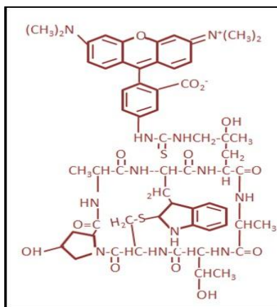
Figure 3.5: Rhodamine Phalloidin
