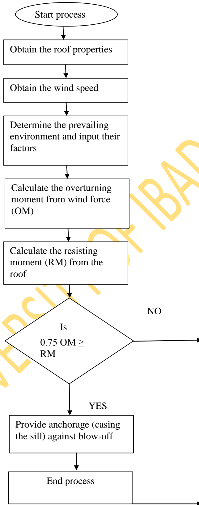
Figure 3.3 Algorithm for the Roof Blow-off Model
