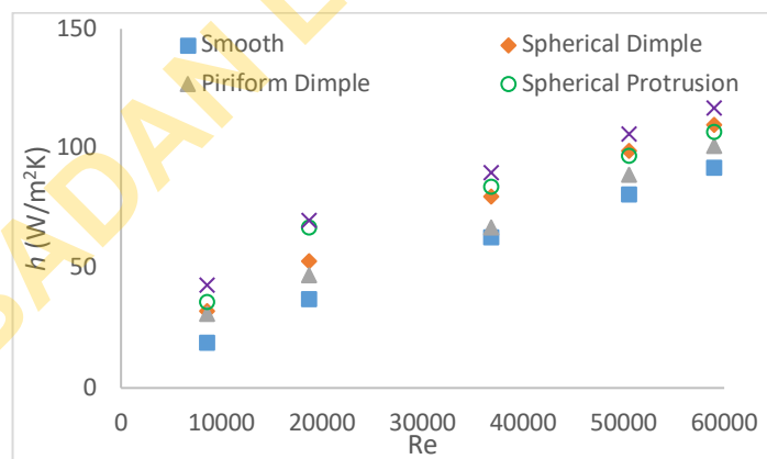
Fig. 8. Heat Transfer Coefficient of test channels
