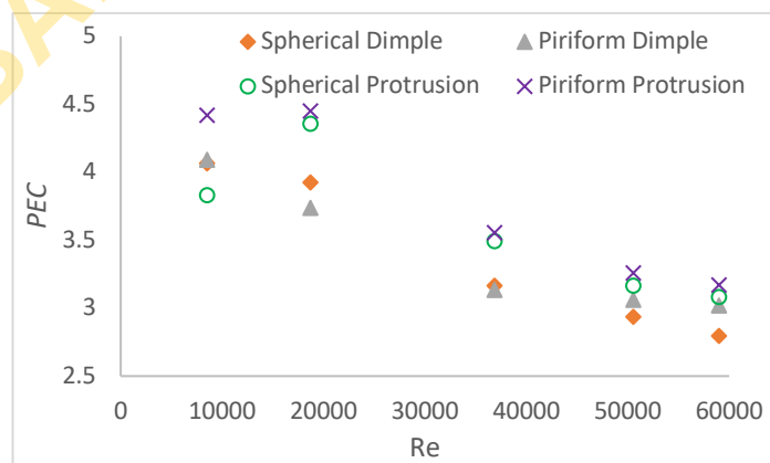
Fig. 13. Overall thermal performance of the dimpled and protruded channels
