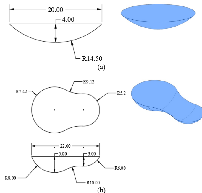
Fig. 2. The geometrical dimensions of the dimples (a) spherical dimple (b) piriform dimple
