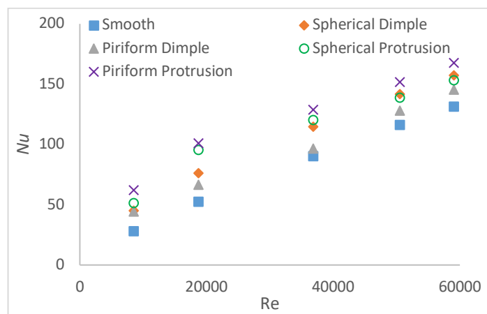
Fig. 9. Nusselt numbers of test channels
