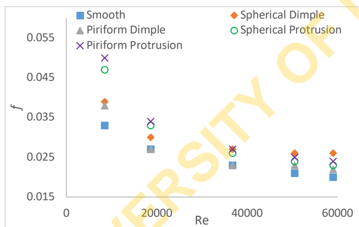
Fig. 11. Friction factors of the test channels
