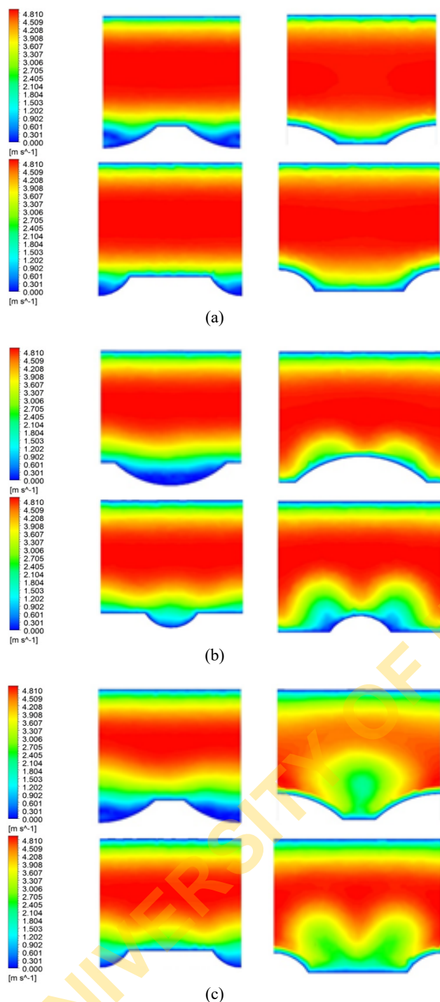
Fig. 6. Velocity plots at transverse cross-sections of spherical-dimpled, spherical-protruded, piriform-dimpled, and piriform-protruded channels (a) 20.0 mm, (b) 122.5 mm, and (c) 230.0 mm of the dimpled/protruded section
