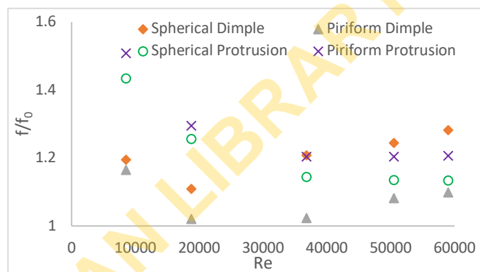
Fig. 12. Normalised friction factor of the dimpled and protruded channels
