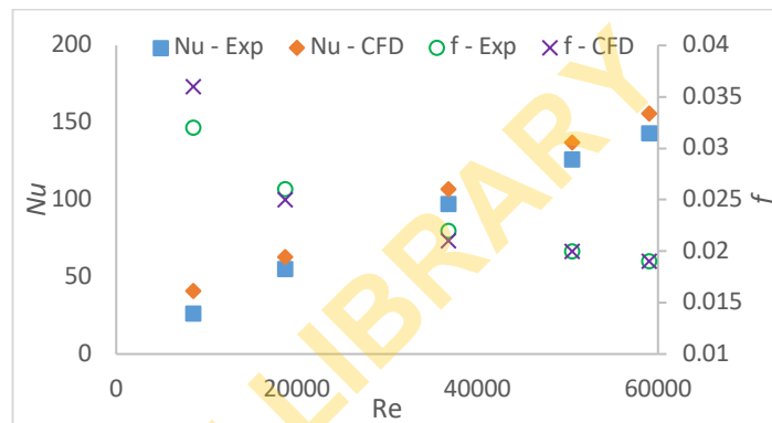
Fig. 5: Nusselt number and friction factor obtained with experimental data
