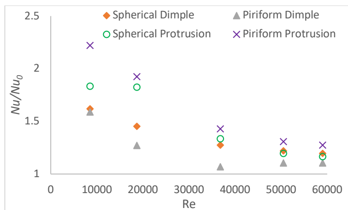
Fig. 10. Nusselt number ratios of the dimpled and protruded channels
