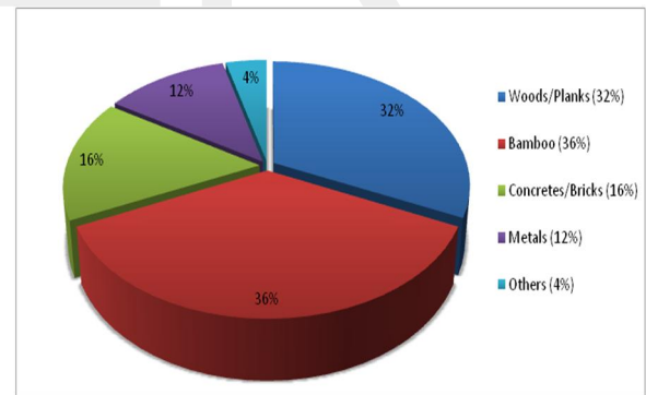
FIGURE 1: PIE CHART SHOWING THE % WEIGHT OF THE VARIOUS WASTE COMPONENTS IDENTIFIED AT CONSTRUCTION SITE A.
