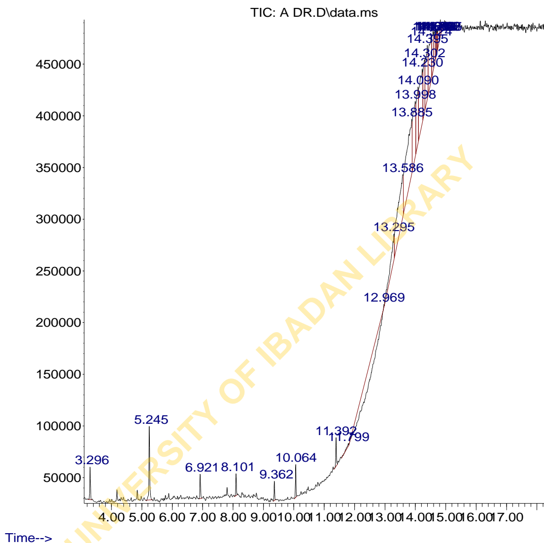
Fig. 5. GC-MS chromatogram of essential oils of methanol extract of M. charantia )
