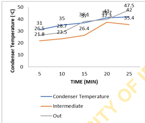
Fig. 7: Variation of Condenser Temperature with Time at an Ambient Temperature of 32°C
