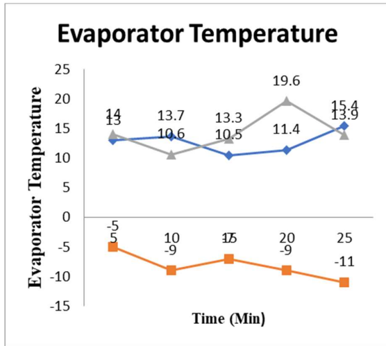
Fig. 6. Variation of Evaporator Temperature with Time at an Ambient Temperature of 32°C
