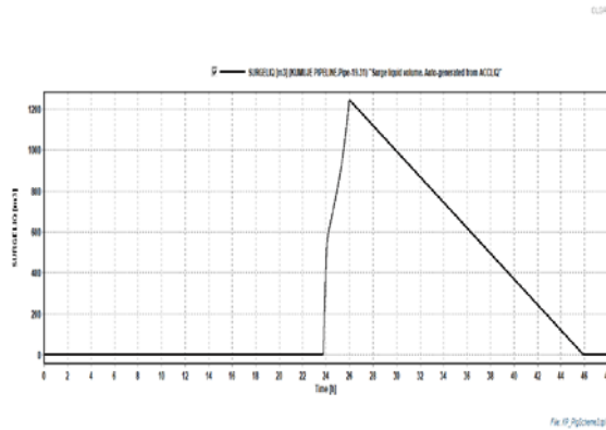
Figure 9: Slug catcher surge volume for pigging scheme 3
