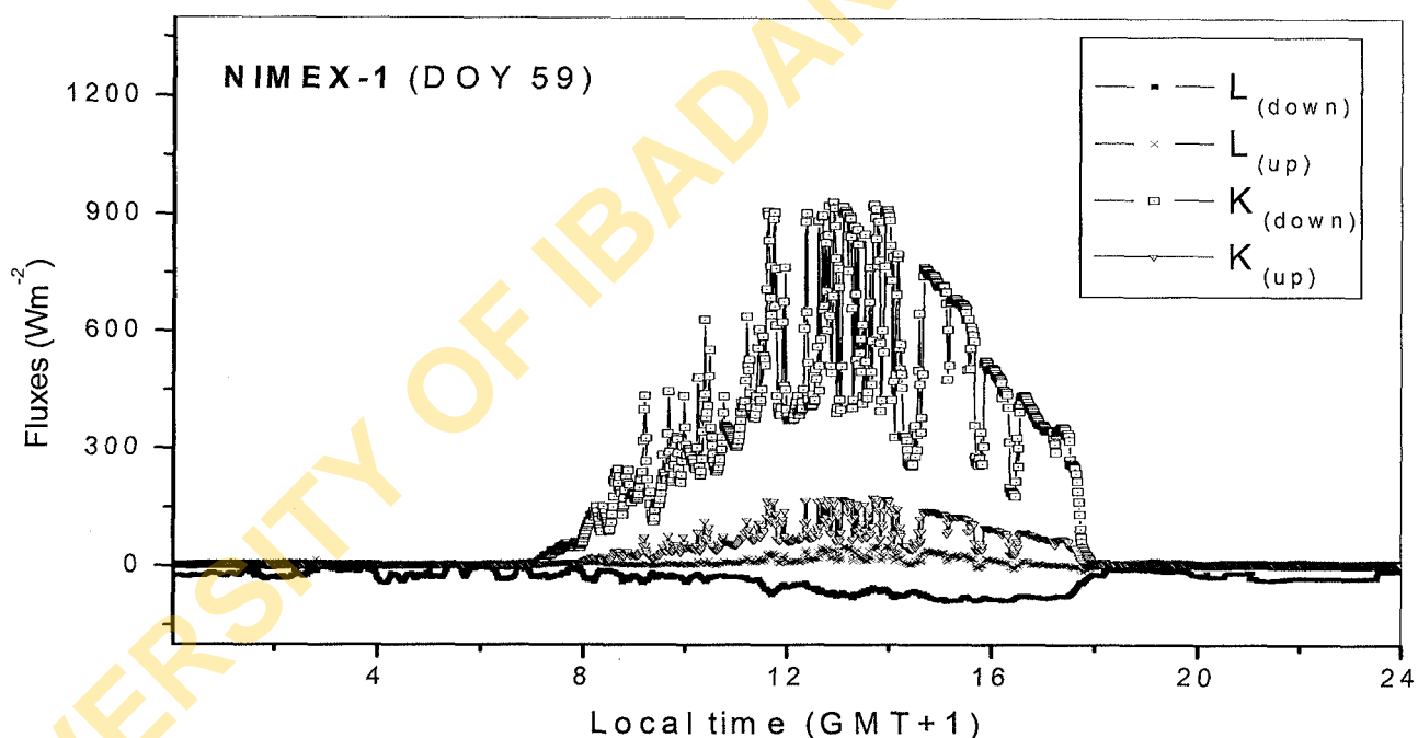
Fig. 10: The radiation components measured, both shortwave and longwave, at the NIMEX-1 site on DOY 59.
