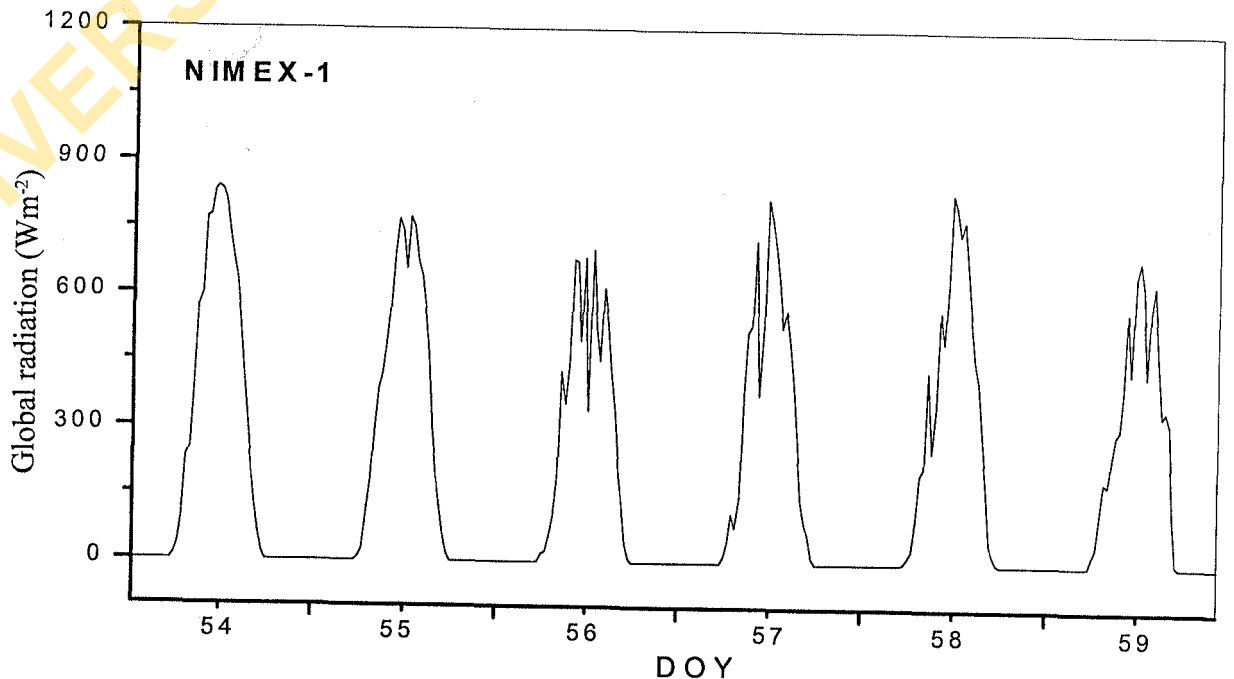
Fig. 8: The diurnal trend of global radiation for DOY 54 to 59 at the NIMEX-1 site
