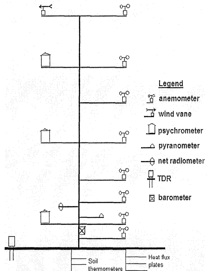
Fig. 2a: Measurement complex M2 (see the text for details)
