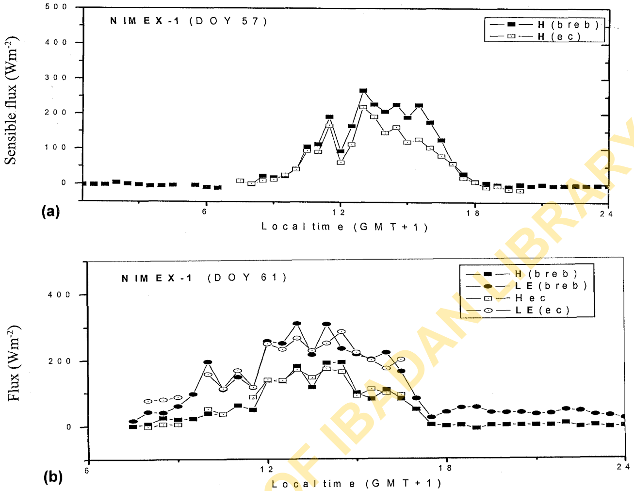
Fig. 5: Comparison of the sensible and latent heat fluxes estimated by BREB method with EC method
