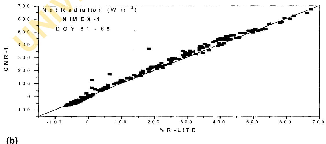
Fig. 9: Comparisons of (a) global and (b) net radiation as measured by SP-LITE and NR-LITE radiometers respectively with a reference net radiometer, CNR-1.
