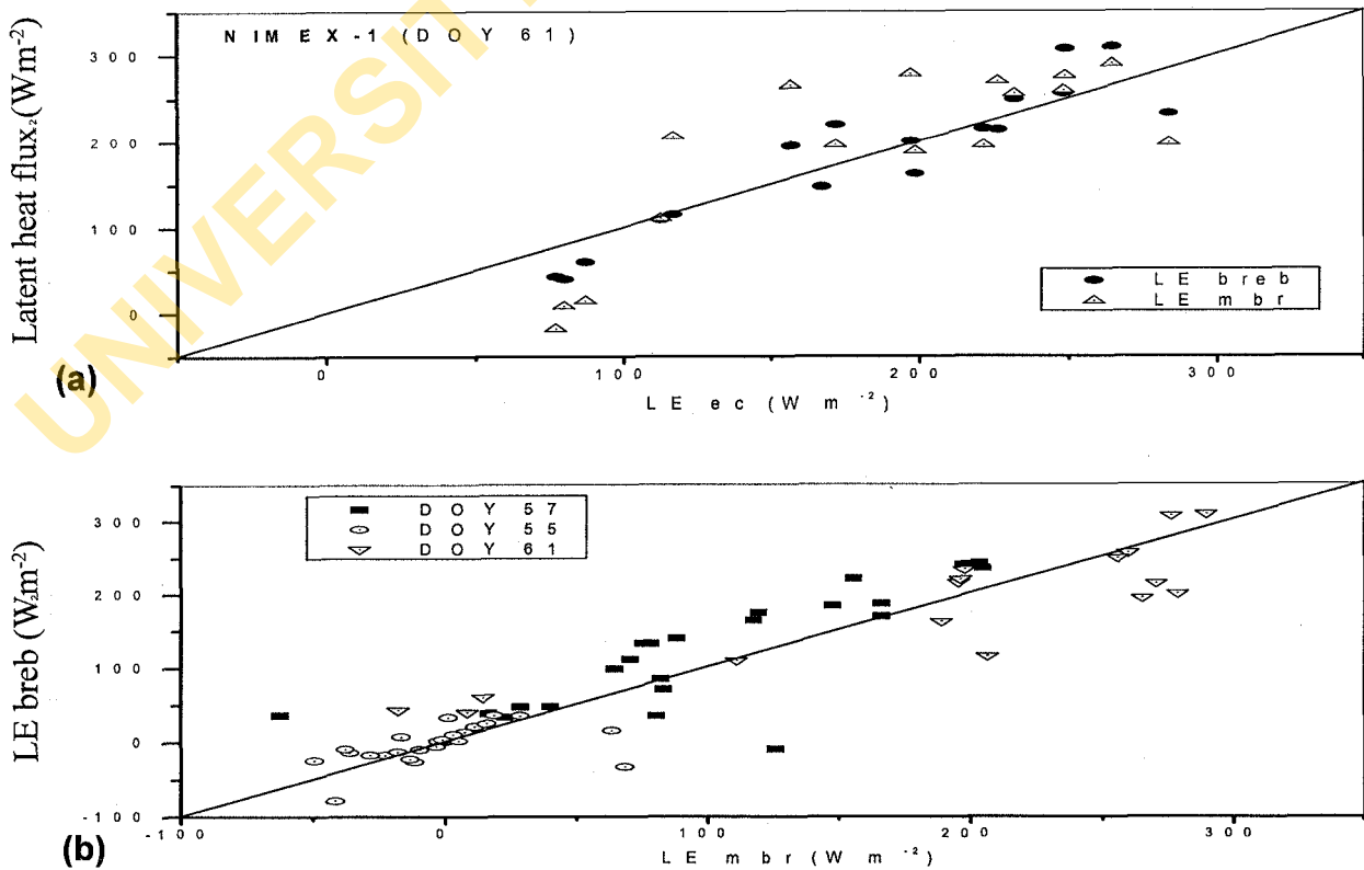
Fig. 6: Comparison of latent heat fluxes estimated by BREB and MBR methods with EC method
