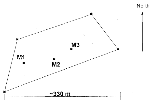
Fig. 1: The positioning of the three complexes: M1, M2 and M3, within the measurement domain
