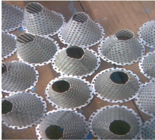
Figure 3: Opening of the frustum
