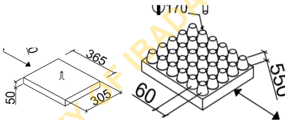
Figure 1: The Mould design
