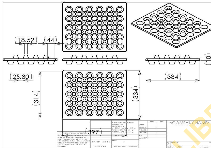
Figure 1: The Mould design
