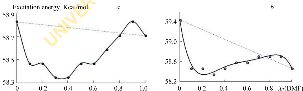
Fig. 3. Variation of E_{12} of AZ-03 (a) and AZ-04 (b) with mole fraction of DMF.
