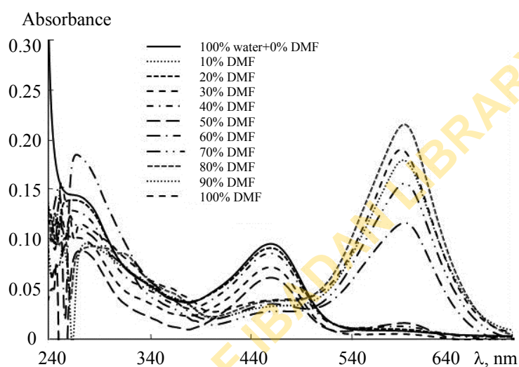
Fig. 2. Electronic absorption spectra of AZ-02 in water:DMF mixtures.
