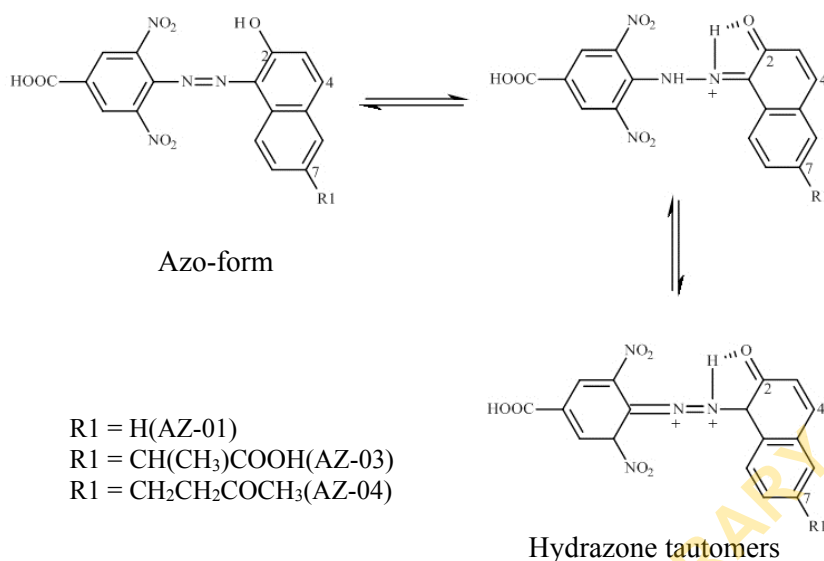
Fig. 1. Azo-hydrazone tautomeric equilibrium in AZ-01, AZ-03, and AZ-04.
