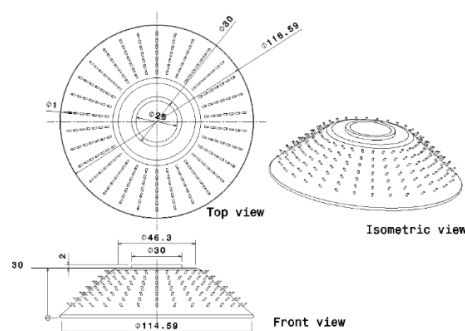
Fig. 8 Blade spike unit drawing
