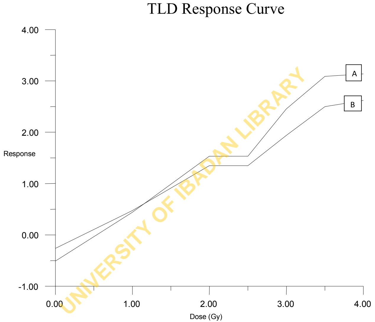
Fig. 1: Calibration Curve for chips A and B
