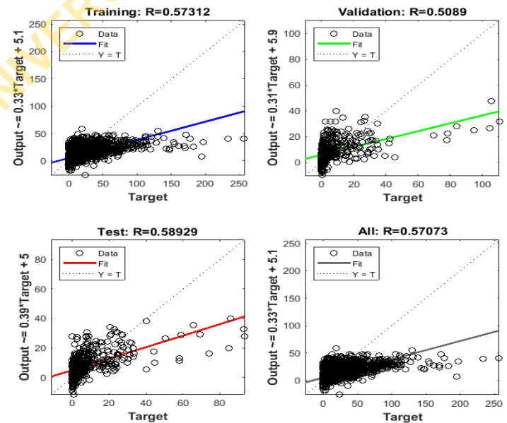
Fig-5: Regression plot of Scaled Conjugate Gradient Predictive Algorithm
