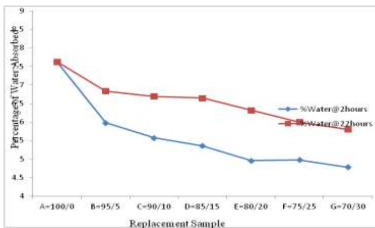
Fig. 4: Water Absorption Test of Cement/ WGP Composite
