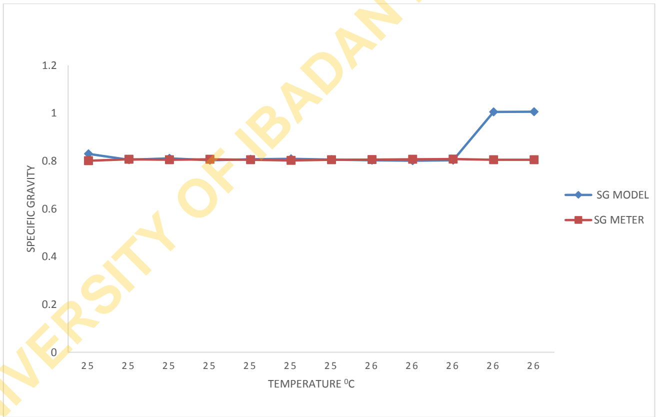
Figure 4.16: Specific Gravity versus Temperature of Petrol/Alcohol mixture
